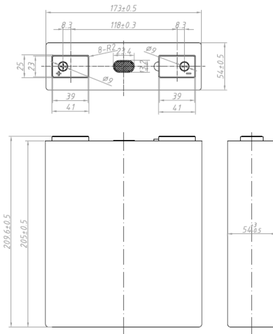
Drawing 1 Appearance and dimension of the battery
